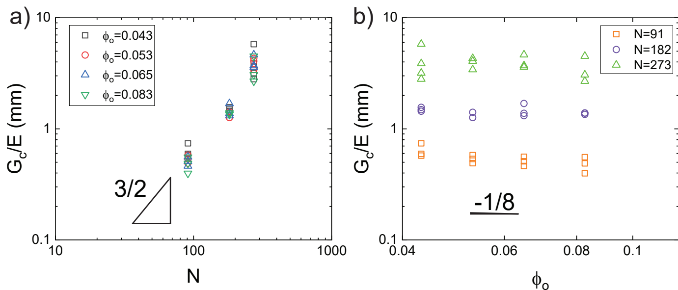
Fig. 2 Plots of the elastofracture length against a) N and b) \phi_o , showing strong agreement with the scaling predictions of Equation (6). Data is taken from pure shear notch tests. 16 Agreement between the data and theoretical scalings shows that altering N is a more effective means of tuning G_c/E .
