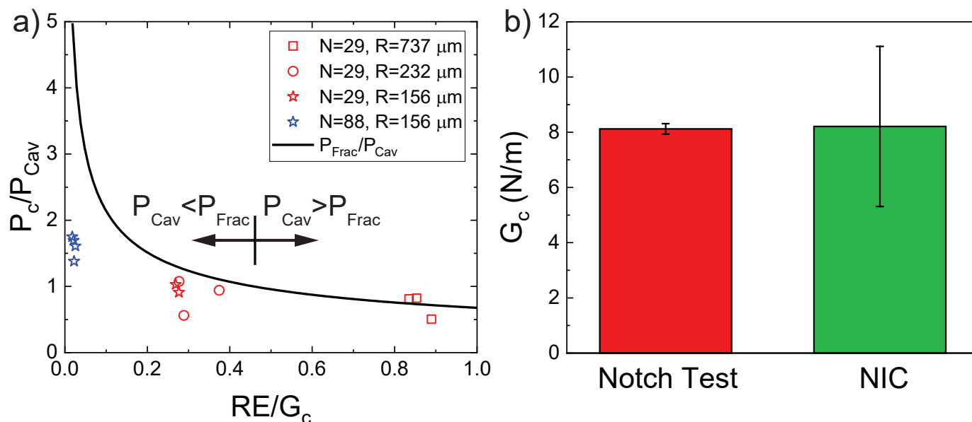
Fig. 4 a) Plot of the experimentally observed critical expansion pressure P_c normalized by P_{Cav} against RE/G_c . The black line represents the point at which fracture is predicted to occur. b) Plot showing the comparison between G_c measured with notch tests by Barney et al. 16 and measured with NIC in this work when RE/G_c \approx 0.84 .
