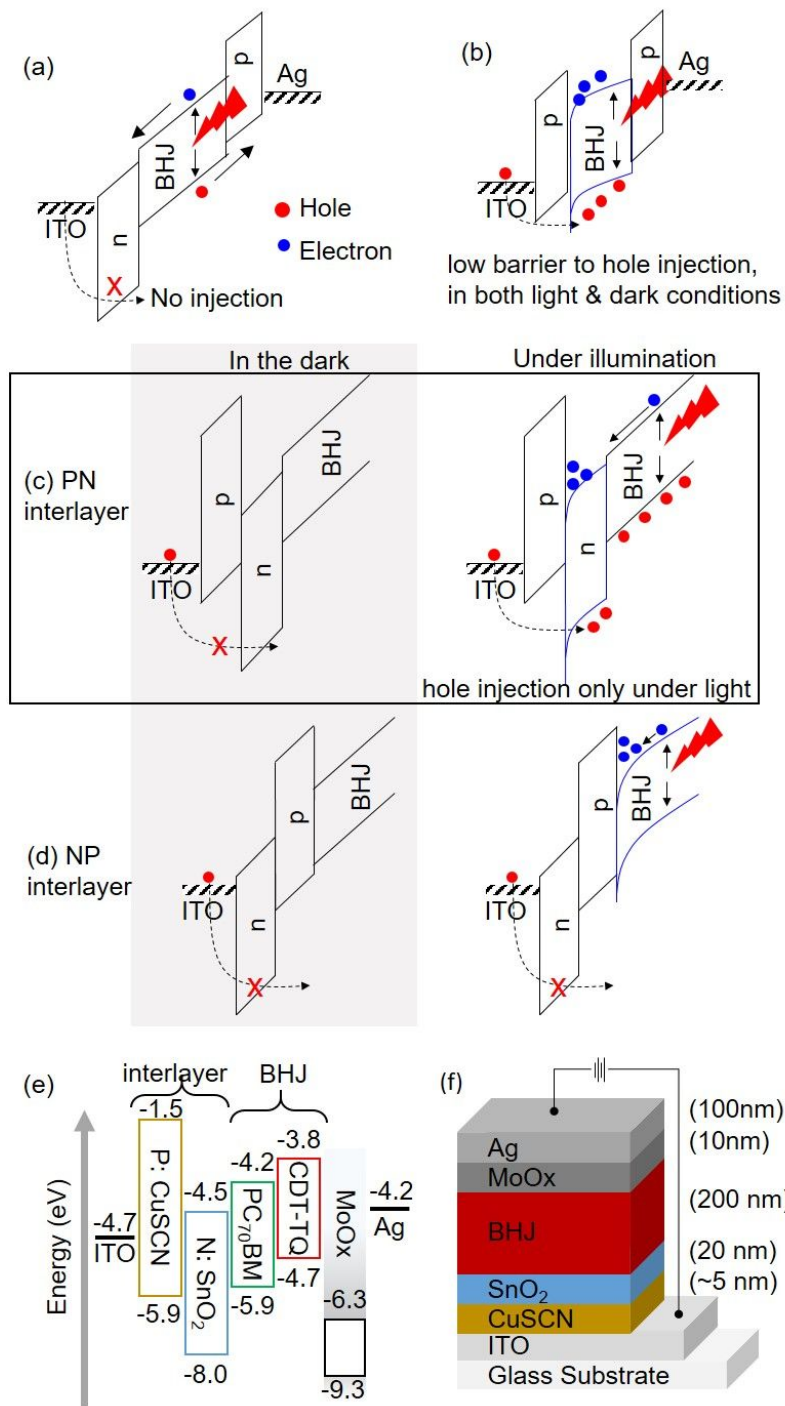
Figure 1. Interlayer designs. Energy diagrams of (a) a conventional photodiode with unipolar charge transporting interlayers and no photomultiplication and (b) a photodiode using a single charge blocking material, which induces photomultiplication but shows high noise current from charge injection in the dark. (c) Changing the interlayer over the ITO electrode to a pn heterojunction bilayer that enables photomultiplication and suppresses dark current. (d)
