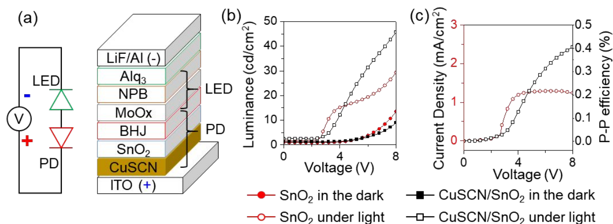
Figure 3. Upconversion imagers with different interlayers in the photodiode stack. The incident light was at an intensity of 5 mW/cm 2 from a 1050 nm light source. (a) Schematics of the upconversion imager with the CuSCN/SnO 2 bilayer. (b) Luminance of the visible light emitted from the imager versus the applied bias. (c) Current density and photon-to-photon upconversion efficiency versus the applied bias.
