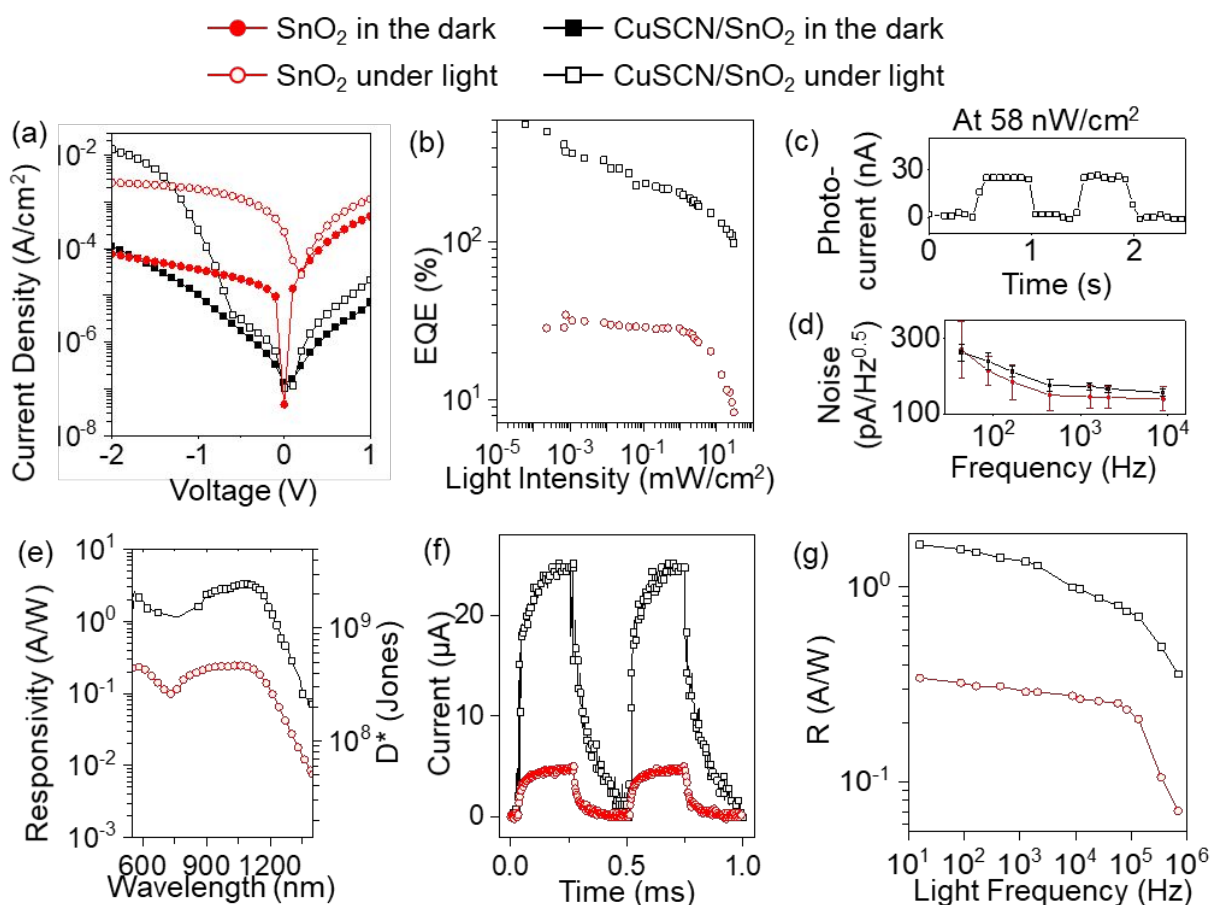
Figure 2. Comparison of the single and bilayer interlayers, with the devices biased at -1.5 V on the Ag electrode. (a) Current density versus applied voltage, measured in the dark and under 9.1 mW/cm 2 illumination from a 1050 nm LED. (b) External quantum efficiency taken at the wavelength of 1050 nm as a function of incident light intensity. (c) Temporal photoresponse
