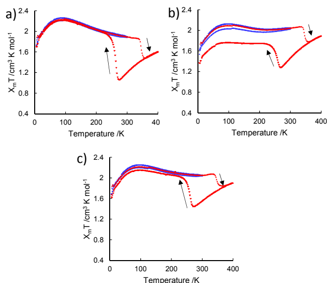
Fig. 4 \chi_m T versus T for (a) 1 /[Co II (MeO-terpy) 2 ], (b) 2 /[Co II (MeO-terpy) 2 ] and (c) 3 /[Co II (MeO-terpy) 2 ] on warming ( \blacktriangle ) and cooling ( \blacktriangledown ). The blue plots indicate the first cycle (from 5 to 300 K) and the red plots indicate the second cycle above the boiling point of water (from 5 to 400 K).
