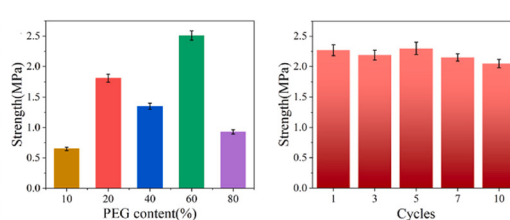
(f) Adhesion strength of BHETA-based adhesive
