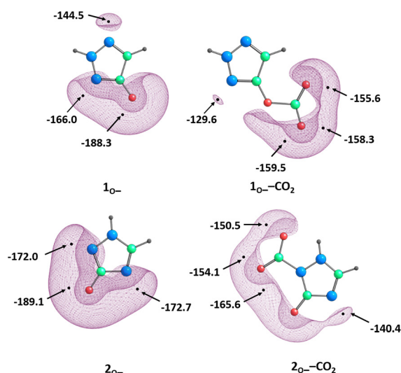
Fig. 5 MESP topography of anions 1 O - , 2 O - and their most stable CO 2 adducts computed at the M06-2X/cc-pVQZ level of theory. Black dots indicate V_{\min} value in kcal mol -1 . Isosurface value: –125 kcal mol -1 . Color key: gray – H, blue – N, green – C, red – O.
