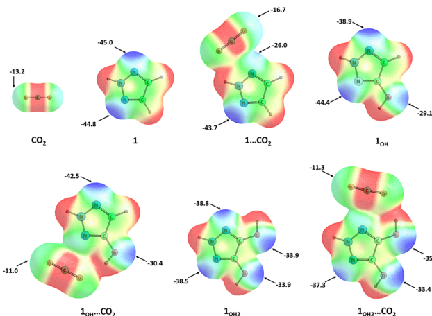
Fig. 3 MESP on the 0.005 a.u. isodensity surface for CO 2 , 1 , 1 OH , 1 OH2 , and their CO 2 complexes. V_{\min} values (kcal mol -1 ) and N...C, O-H...O distances (Å) at the M06-2X/cc-pVQZ level of theory. Color gradient: blue (electron-rich) to red (electron-deficient).
