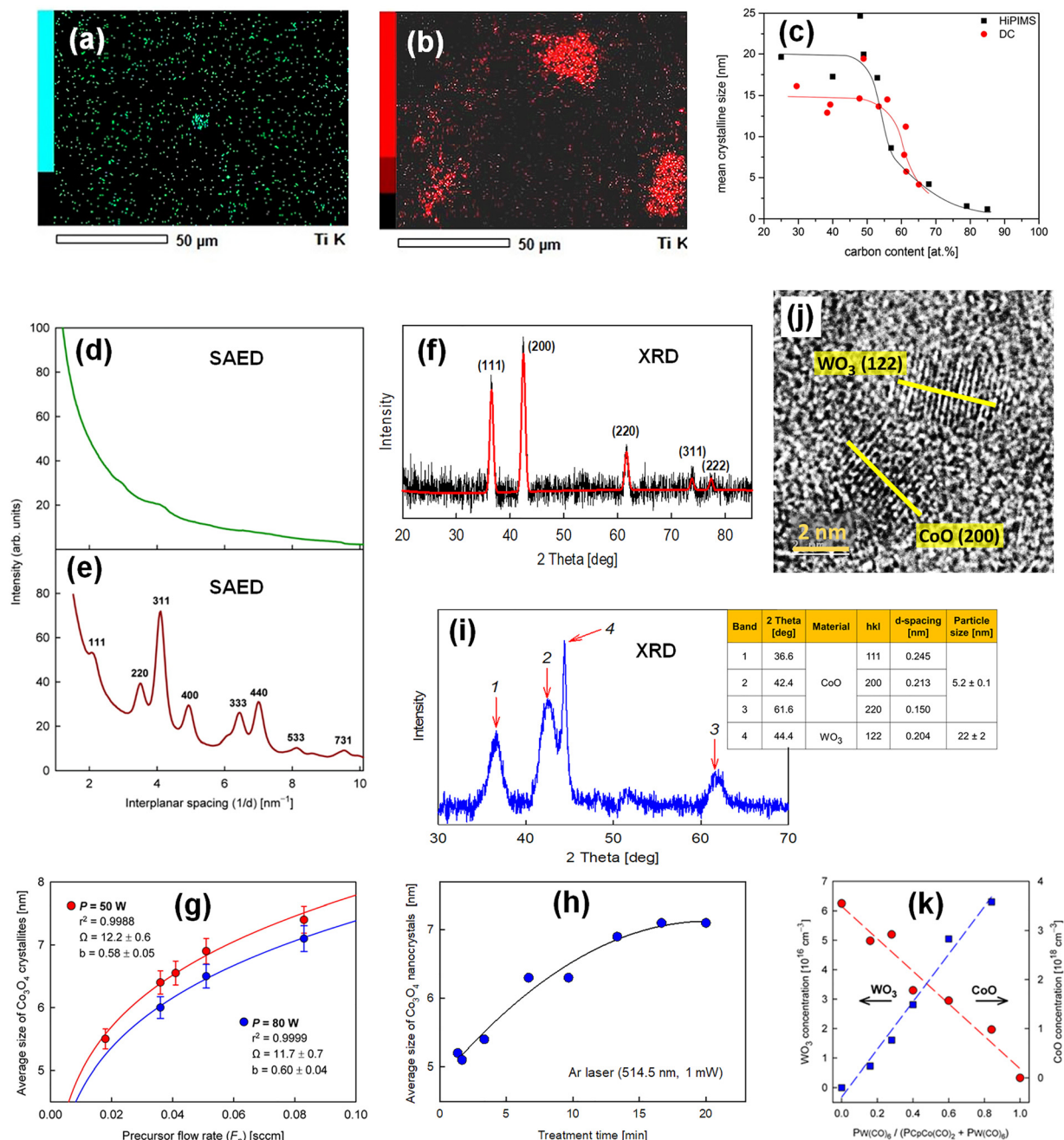
Fig. 5 Nanostructure of thin-film nanocomposites deposited by cold plasma methods: (a) and (b) Ti atomic intensity maps for films composed of \text{TiO}_2 nanoparticles embedded in a silicon-carbon-oxide matrix, deposited by a hybrid PECVD + sputtering method using a reaction mixture containing 20% and 50% oxygen, respectively. 63 (c) TiC nanocrystallite size as a function of carbon content in films deposited by a hybrid PECVD + sputtering method using a Ti target and varying acetylene content in a \text{C}_2\text{H}_2/\text{Ar} reaction mixture; two deposition modes – direct-current magnetron sputtering (DC) and high-power impulse magnetron sputtering (HiPIMS) – were applied, reproduced from ref. 64 with permission from Elsevier, copyright 2017. (d) and (e) Electron diffraction (SAED) patterns of \text{CoO}_x -based films fabricated by PECVD, as-deposited (amorphous structure) and after thermal treatment in oxygen ( \text{Co}_3\text{O}_4 structure), respectively. 118 (f) XRD pattern of the same \text{CoO}_x -based film after thermal treatment in argon ( \text{CoO} structure). 117 (g) Dependence of the \text{Co}_3\text{O}_4 nanocrystalline size on the \text{CpCo}(\text{CO})_2 precursor flow rate and discharge power for films deposited by PECVD and subsequently thermally treated in oxygen; the curves represent a model describing the nucleation and growth of these nanocrystallites. 118 (h) Regulation of the \text{Co}_3\text{O}_4 nanocrystallite size using an argon laser to precisely control the thermal treatment time for films deposited analogously to those in (g), reproduced from ref. 26 with permission from Elsevier, copyright 2019. (i) XRD pattern of a nanocomposite film containing \text{CoO} and \text{WO}_3 nanoparticles in a carbon matrix fabricated by PECVD co-deposition, and (j) HRTEM micrograph revealing fragments of crystallographic planes that correspond to these nanoparticles, reproduced from ref. 100 with permission from Wiley-VCH, copyright 2025. (k) Concentrations of \text{CoO} and \text{WO}_3 nanoparticles as a function of precursor partial pressures for films co-deposited by PECVD using \text{CpCo}(\text{CO})_2 and \text{W}(\text{CO})_6 ; the plot is based on numerical data reported in ref. 100.
