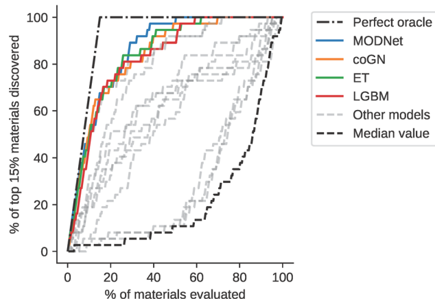
Fig. 5 Discovery curves for the benchmarked models on the top 15% of compounds in the holdout set.
