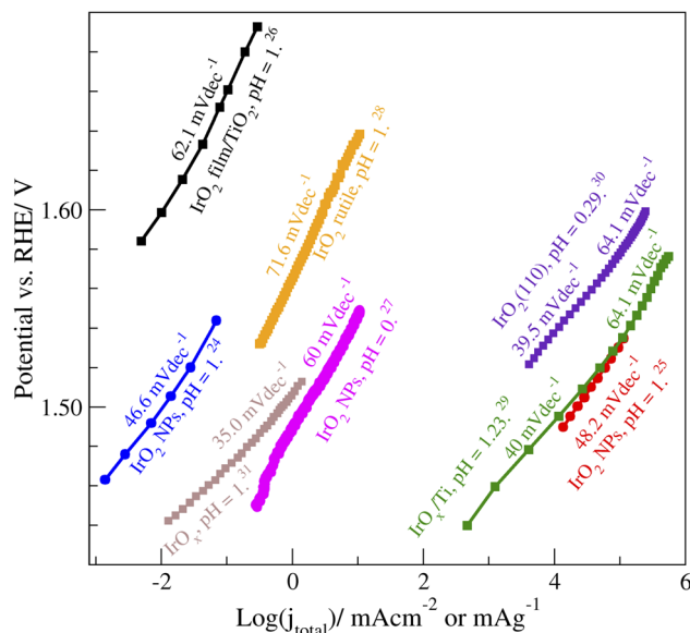
Fig. 1 Experimental Tafel plots for OER on \text{IrO}_x -based catalysts in acidic conditions. Square and circle symbols represent films and nanoparticles (NPs), respectively. 24–31 Note that the reported current densities ( j_{\text{total}} ) vary in their normalization, making the direct comparison of j_{\text{total}} unjustified. This does not affect the highlighted Tafel slope values.
