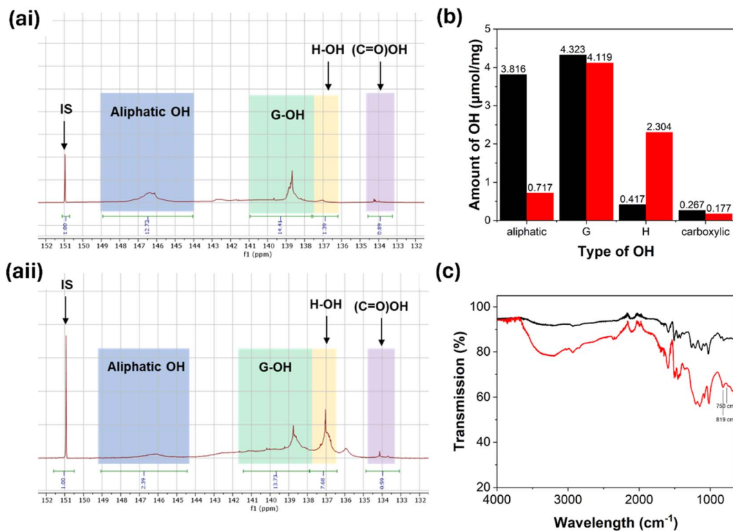
Fig. 10 (a) Liquid-state 31 P NMR collected of phosphitylated (i) KL and (ii) and KL-Ph. (b) Graph summarising the amounts of each different OH group present in KL before (black) and after (red) phenolation. (c) FTIR spectra of KL (black) and KL-Ph (red).
