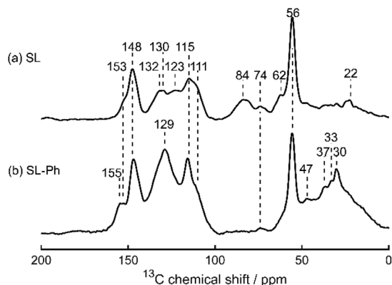
Fig. 11 Solid-state 13 C CP MAS NMR spectra of (a) Sonichem lignin and (b) phenolated Sonichem lignin. Chemical shift values (in ppm) of each peak are indicated.
