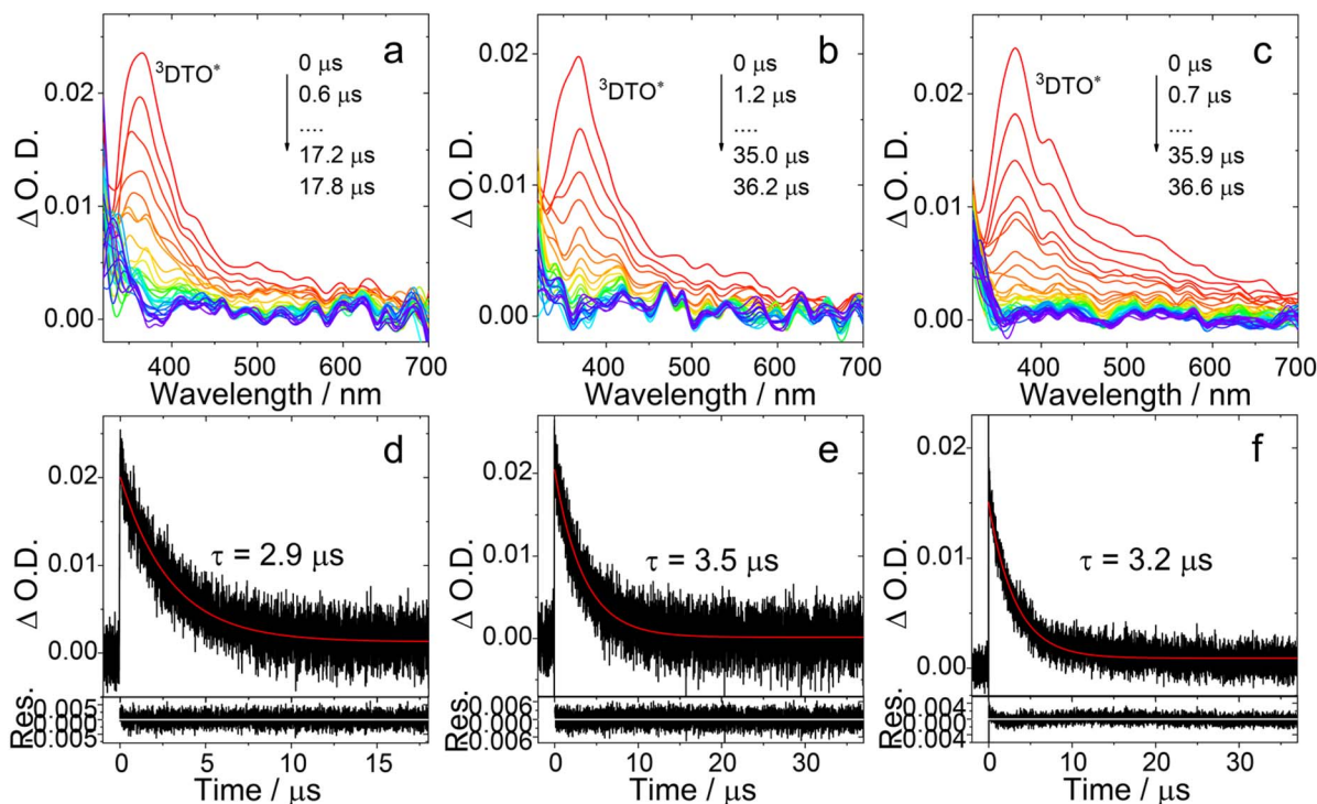
Fig. 7 Nanosecond transient absorption spectra of (a) PTZ-O-DTO, (b) PTZ-O 2 -D 2 O and (c) DPTZ-O-D 2 O. Decay traces of (d) PTZ-O-DTO, (e) PTZ-O 2 -D 2 O and (f) DPTZ-O-D 2 O at 370 nm after pulsed laser excitation at 355 nm. c = 2.0 \times 10^{-5} M in deaerated TOL, 25 °C.
