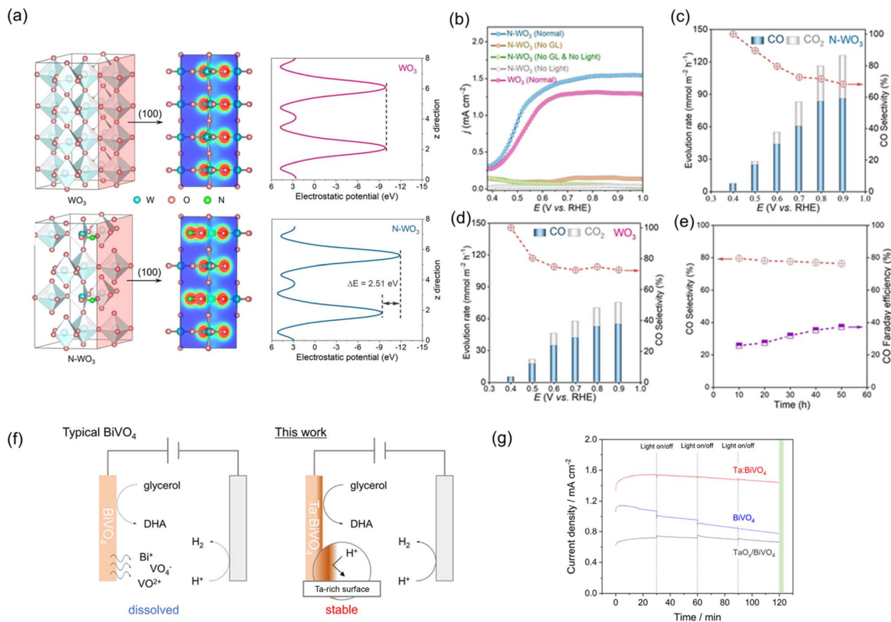
Fig. 9 (a) Calculated isosurface of electron density and electrostatic potential of WO 3 and N-WO 3 . (b) LSV curves of N-WO 3 in the absence and presence of glycerol under dark or light irradiation. Evolution rate and CO selectivity of (c) N-WO 3 and (d) WO 3 . (e) Long-term stability of PEC glycerol oxidation toward CO generation at 0.6 V RHE . Reproduced with permission. 110 Copyright 2022, John Wiley and Sons. (f) Schematic of PEC glycerol oxidation over BiVO 4 and Ta:BiVO 4 in acidic medium. (g) Long-term stability of PEC glycerol oxidation over BiVO 4 , Ta:BiVO 4 , and TaO x /BiVO 4 at 1.0 V RHE . Reproduced with permission. 112 Copyright 2022, American Chemical Society.
