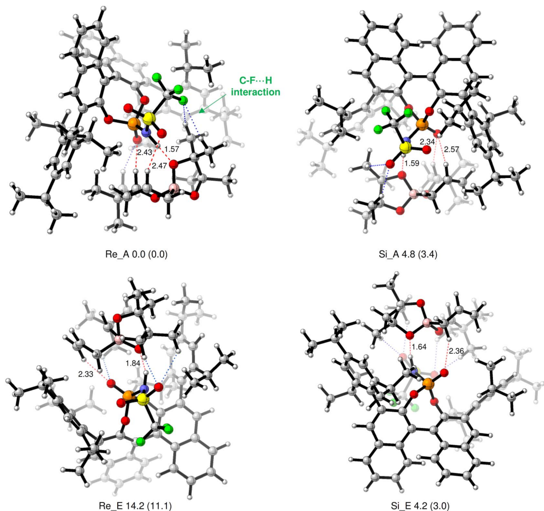
Fig. 3 Optimized transition states of Re_A, Re_E, Si_A, and Se_E at the M06-2X/6-31G(d) level of theory. Bond lengths are given in Å. Values enclosed in parentheses are energies relative to "Re_A" calculated by MN15/6-31g(d)+SDM (toluene). Energy differences are given in kcal mol -1 . See the ESI† on page S38 in detail.
