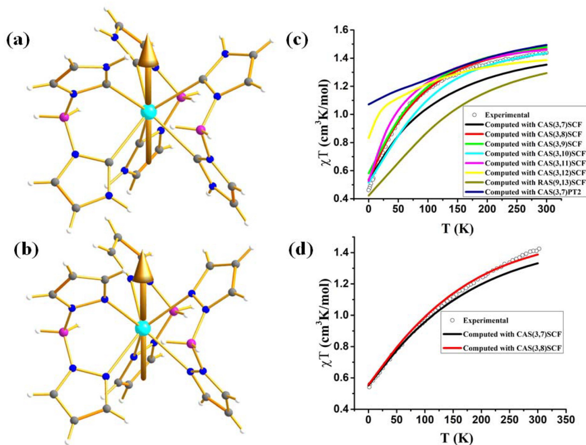
Fig. 9 Molecular structure of the complex (a) [\text{U}(\text{Bc}^{\text{Me}})_3] ( 13 ) (b) [\text{U}(\text{Bp}^{\text{Me}})_3] ( 14 ). Colour code: U (cyan), B (pink), N (blue), C (grey), H (white). Experimental vs. computer temperature-dependent magnetic susceptibility of (c) 13 (d) 14 with several active spaces.
