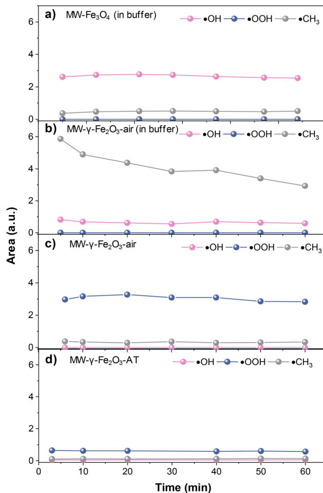
Fig. 4 Effect of the buffer and the oxidation of the NPs on the free radical formation measured at \text{pH} = 4.8 . (a) \text{Fe}_3\text{O}_4 in buffer, (b) MW- \gamma\text{-Fe}_2\text{O}_3 -air in buffer, (c) MW- \gamma\text{-Fe}_2\text{O}_3 -air measured without buffer and (d) MW- \gamma\text{-Fe}_2\text{O}_3 oxidized by an acidic treatment (AT) measured without buffer.
