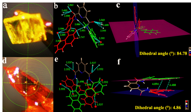
Fig. 2 Crystal photographs (a) and (d), hydrogen bonding (b) and (e), and dihedral angle (c) and (f) of \text{H}_4\text{L}^2\text{-}\gamma and \text{H}_4\text{L}^2\text{-r} Crystal, respectively; reproduced from ref. 57 with permission from RSC, Copyright 2022.
