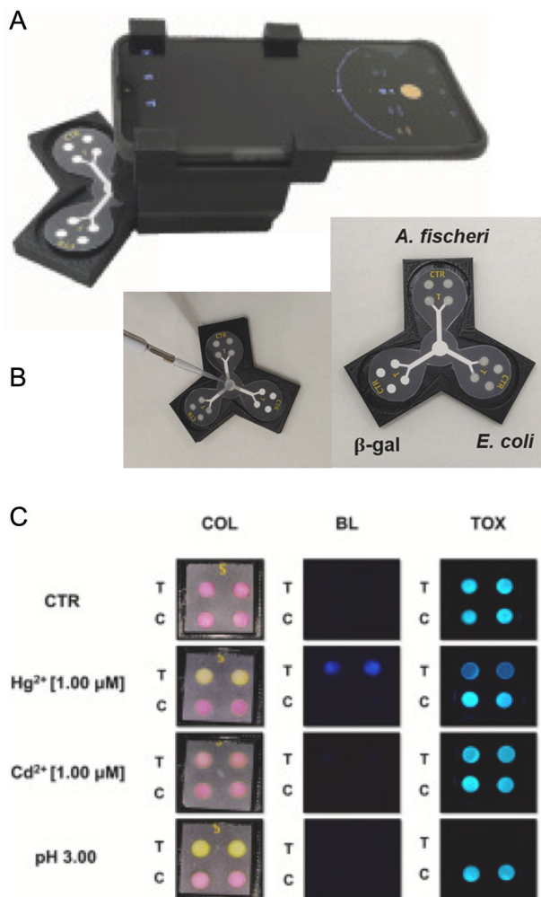
Fig. 40 Smartphone-based device for a dual colorimetric and bioluminescent detection of Hg^{2+} (aq). Photographs of (A) the device and (B) the three-leaf test strip system. The test used a chromogenic reaction catalyzed by \beta -galactosidase and two bioluminescent bacterial strain reporters ( E. coli and A. fischeri ). (C) Brightfield (COL) and BL images of the test strip responses to Hg^{2+} , Cd^{2+} and low pH. Adapted with permission from ref. 549 Copyright 2021 Elsevier B.V.
