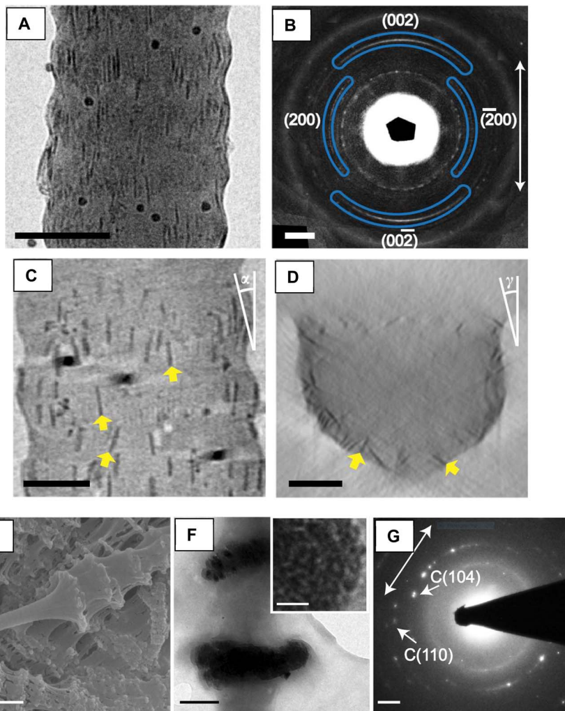
Fig. 23 Xu et al. 114 studied the effect of confinement on crystal growth in collagen by using XRD to determine the voids in collagen are cylindrical pores with diameters of around 2 nm. (A) and (B) In addition to HAp (not shown here), they also demonstrated the concept of confinement with lepidocrocite, \gamma -FeOOH, which also has an anisotropic lattice structure (orthorhombic). (C) and (D) Tomographic reconstruction with an averaging of ten y - and z -slices. The orientations of some \gamma -FeOOH platelets are highlighted by yellow arrows in (C). (E)–(G) They found that \text{CaCO}_3 produced a mix of calcite and vaterite (not shown here), and with a sustained granular texture, they showed no preferential orientation. Interestingly, their intrafibrillar calcite produced orthogonal bulges similar to what we had observed in our first \text{CaCO}_3 collagen study. It would be interesting if someone could produce intrafibrillar aragonite, because it normally grows as anisotropic needles. Reproduced from ref. 114, Copyright © 2020, The Authors.
