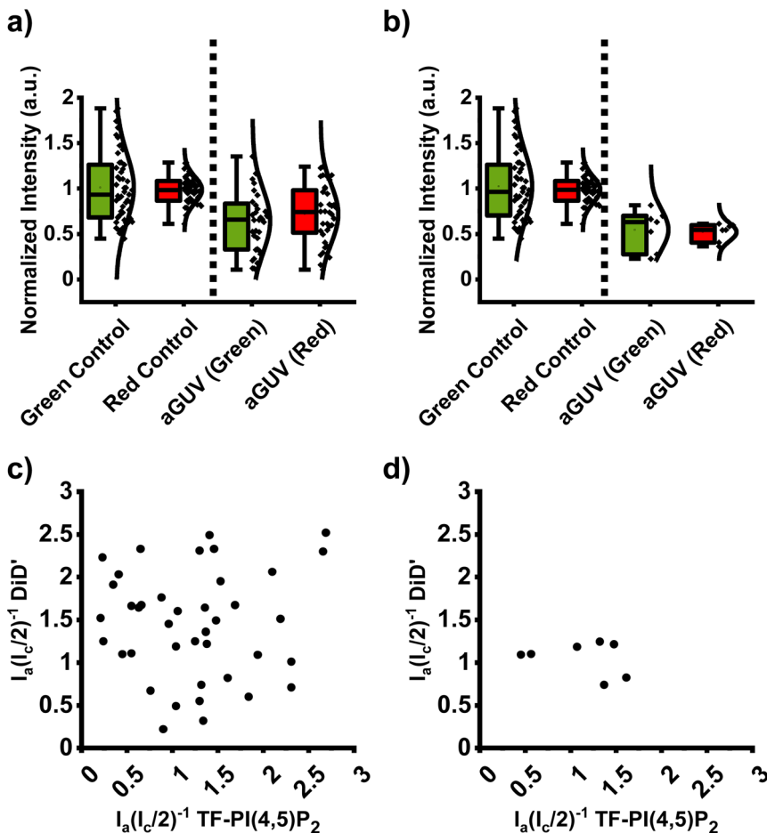
Fig. 4 DOPC/DiD (inner leaflet, red channel):DOPC/PI(4,5) \text{P}_2 /TF-PI(4,5) \text{P}_2 (outer leaflet, green channel) asymmetric giant unilamellar vesicles prepared using 6 mM \text{Mg}^{2+} as the hemifusion initiator. (a) Comparison of sGUV controls for the green (TF-PI(4,5) \text{P}_2 ; N = 49 ) and red (DiD'; N = 46 ) channels to the corresponding fluorescence channels of imaged aGUVs ( N = 40 ) across 5 separate experiments. (b) the range-passing aGUVs from the samples presented in (a). (c) Cross-correlation of the two channels for individual aGUVs. A "perfect" aGUV would be found at the data point (1,1) which corresponds to a completely exchanged outer leaflet and no artifacts like multi-lamellarity. (d) Cross-correlation of the two channels for the range-passing aGUVs. sGUV buffer: 97 mM NaCl, 100 mM KCl, 1 mM \text{Na}_2\text{EDTA} , 25 mM HEPES pH = 7.4 buffer. aGUV buffer after hemifusion: 97 mM NaCl, 100 mM KCl, 7 mM \text{Na}_2\text{EDTA} , 25 mM HEPES pH = 7.4 buffer. The controls displayed in (a) and (b) are the same experiments and are reproduced for comparison.
