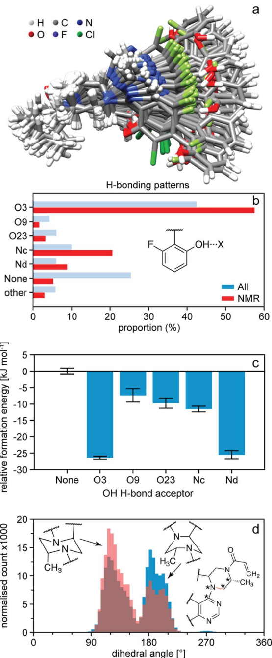
Fig. 8 The structure of amorphous AZD4625. 165 (a) Superposition of 100 conformations randomly sampled from the NMR set, and aligned on atoms Nb–C5–C4–Na. (b) Proportions of different hydrogen bond acceptors bonded to the OH group of AZD4625 in all local molecular environments (blue) and in the NMR set (red). (c) Computed relative formation energies of the local molecular environments in the NMR set for different hydrogen bond acceptors bonded to the OH proton. The zero is set to be the mean formation energy of intermolecular complexes where no hydrogen bonding acceptor is
