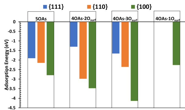
Fig. 1 Adsorption energies of arsenate species in different binding configurations on the stoichiometric \{111\} , \{110\} , and \{100\} surfaces of \text{CeO}_2 . 5OAs denotes five-fold coordinated As species, and 4OAs-1O surf , 4OAs-2O surf , 4OAs-3O surf denote four-fold coordinated As species adsorbed in monodentate, bidentate and tridentate configurations, respectively.
