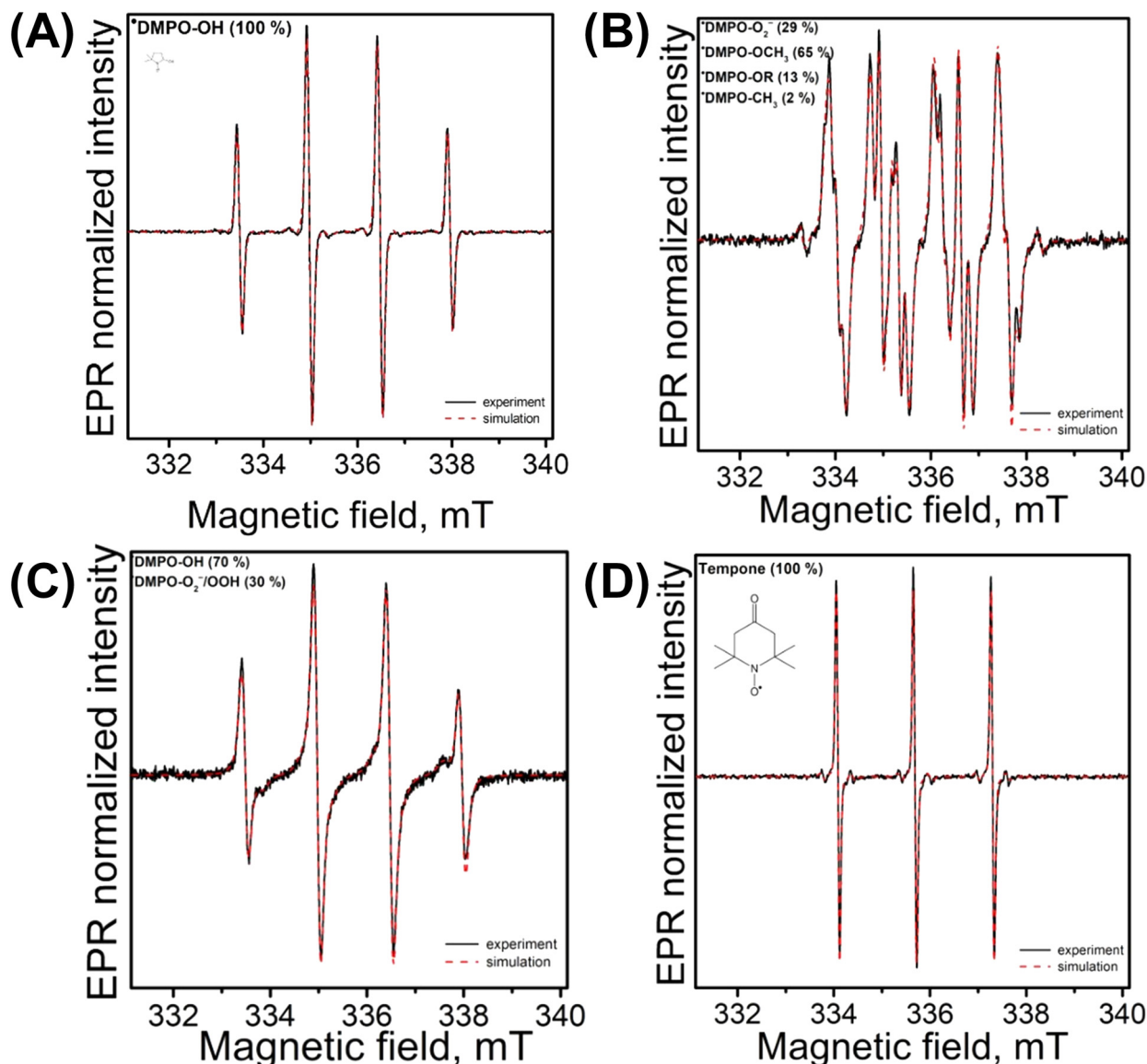
Fig. 7 Experimental (black) and simulated (red) EPR spectra (SW = 9 mT) obtained upon LED@365 nm exposure (irradiance 17 \text{ mW cm}^{-2} ; exposure 300 s) of the aerated \text{TiAP}_{0.1\text{Fe}} suspensions in the presence of (A) spin trap DMPO in water, (B) spin trap DMPO in DMSO, (C) spin trap DMPO in water in the presence of \text{H}_2\text{O}_2 (0.7% vol.) and (D) sterically hindered amine TMPO in water ( \text{TiAP}_{0.1\text{Fe}} concentration 0.2 \text{ mg mL}^{-1} ; c_{0,\text{DMPO}} = 0.042 \text{ M} ; c_{0,\text{TMPO}} = 0.010 \text{ M} ).
