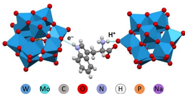
Fig. 11 A fragment of the crystal structure of (HTRP) 3 [PW 12 O 40 ] 1 ·5H 2 O with indication of strong interactions responsible for electron and proton transfer. 34
