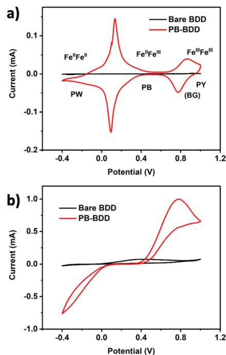
Fig. 3 Cyclic voltammetry of solutions containing (a) 0.1 M KCl and 0.1 M HCl and (b) PBS (pH 7.1.4) containing 100 mM \text{H}_2\text{O}_2 . WE: bare BDD (black line) and PB-BDD (red line). Scan rate 0.1 \text{ V s}^{-1} .
