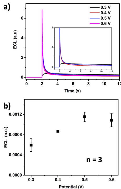
Fig. 2 (a) ECL by chronoamperometry of 0.5 mM luminol in 0.1 M PBS (pH 7.4) in the presence of 10 \mu\text{M} \text{H}_2\text{O}_2 at different potentials; (b) integrated ECL signals vs. applied potential. WE: BDD.
