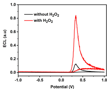
Fig. 1 ECL signal by cyclic voltammetry of 0.5 mM luminol in 0.1 M PBS (pH 7.4) in the absence (black line) and in the presence (red line) of 10 mM \text{H}_2\text{O}_2 , scan rate 0.1 \text{ V s}^{-1} . WE: BDD.
