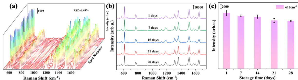
Fig. 5 (a) Reproducibility for R6G detection by \text{Fe}_3\text{O}_4@\text{CoNi LDH}@\text{Ag} NP substrate; (b) SERS spectra of 1 \times 10^{-6} mol per L R6G on the \text{Fe}_3\text{O}_4@\text{CoNi LDH}@\text{Ag} NP substrate recorded every 7 days; and (c) storage time on the SERS response of the \text{Fe}_3\text{O}_4@\text{CoNi LDH}@\text{Ag} NP substrate toward R6G ( \text{mol L}^{-1} ) at 612 \text{ cm}^{-1} .
