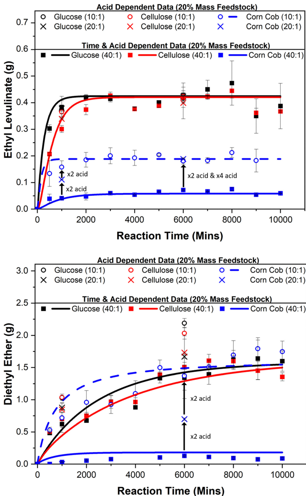
Fig. 5 Ethyl levulinat (g) and diethyl ether (g) produced from the sulphuric acid-catalysed ethanolytic of glucose, cellulose, and corn cob (5, 10, and 20 mass percent) for three different feedstock-to-acid ratios (10 : 1, 20 : 1, and 40 : 1) at 150 °C. Full time-dependent data sets are produced for a feedstock-to-acid ratio of 40. An additional time-dependent data set was produced for corn cob only at a feedstock-to-acid ratio of 10 : 1. At 1000 and 6000 minutes, reactions are performed varying the feedstock-to-acid ratio (10 : 1, 20 : 1, and 40 : 1) to determine the acid dependence of the process in both the kinetic and steady-state phases. The square, cross, and circle data points represent experimental data, and the lines represent the chemical kinetic model.
