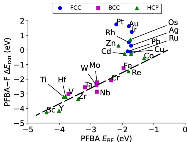
Fig. 5 PFBA binding vs. \Delta E_{\text{rxn}}^{\text{PFBA-F}} for the removal of a \text{F} from a \text{C}_\alpha carbon on transition metal surfaces. The black dashed line represents a linear fit to the data for the carbo binding mode ( \Delta E_{\text{rxn}}^{\text{PFBA-F}} = 0.57E_{\text{BE}}^{\text{PFBA}} + 1.06 , R^2 = 0.90 ). No stable solution exists for the linear regression of the flat binding mode.
