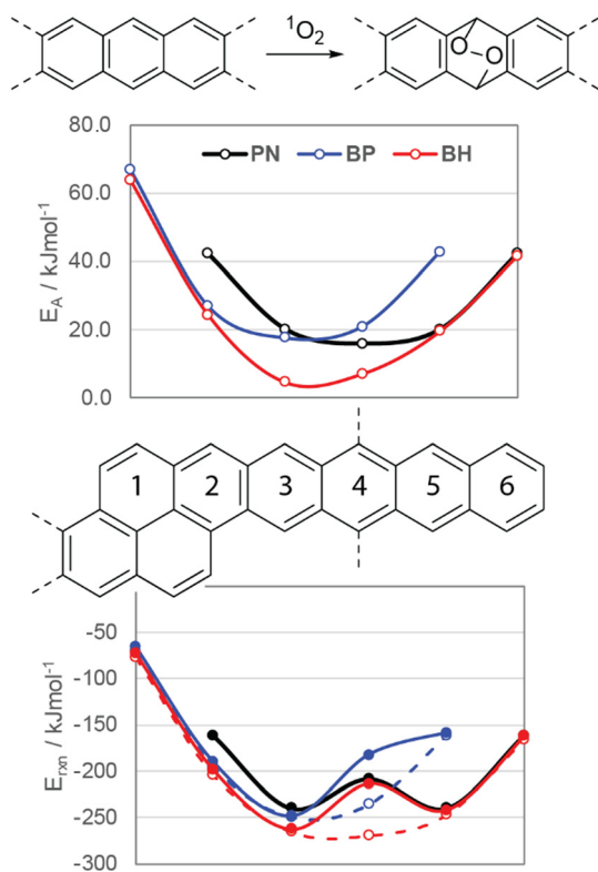
Fig. 6 (top) Activation energies and (bottom) reaction energies of bisacenes with singlet oxygen at different ring positions. Open circles are without the silylethynyl groups, and filled circles are with these groups included. All energies computed with M06-2X/cc-pVTZ.
