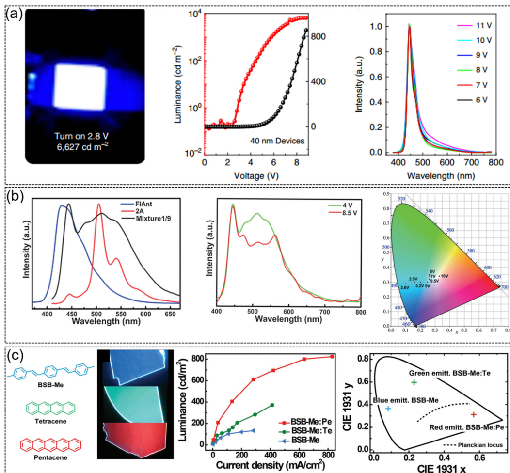
Fig. 9 Representative applications in OLEDs. (a) Strong blue emission from OLEDs based on DPA ( 2 \text{ mm} \times 2 \text{ mm} ), current density–voltage–luminance characteristics of the OLEDs and EL spectra operated at different voltages. Reproduced with permission. 39 Copyright 2015, Springer Nature. (b) EL spectra in OLEDs based on FlAnt, 2A, and mixture1/9, EL spectra of mixture1/9 at 4 and 8.5 V and CIE coordinates at different driving voltages in OLED devices based on mixture1/9. Reproduced with permission. 66 Copyright 2016, John Wiley and Sons. (c) Chemical structures and top-view photographs of BSB-Me, BSB-Me:Te, and BSB-Me:Pe organic crystals under UV-light irradiation, EL performance of BSB-Me, BSB-Me:Te, and BSB-Me:Pe single-crystal-based OLEDs and corresponding 1931 CIE coordinate diagrams of blue, green, and red light emission with CIE coordinates of (0.56, 0.31), (0.23, 0.59), and (0.08, 0.36), respectively. Reproduced with permission. 137 Copyright 2017, John Wiley and Sons.
