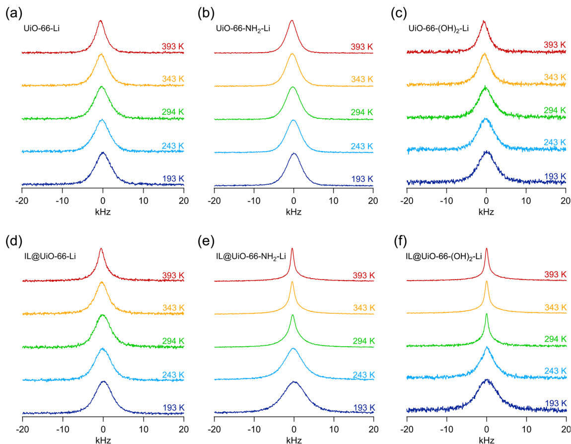
Fig. 5 Variable-temperature ^7\text{Li} NMR (spin quantum number I = 3/2 ) lines acquired in a magnetic field B_0 of 7 T for which the ^7\text{Li} NMR resonance frequency is 116.59 MHz. The width of the NMR line correlates with the jump rates of the probed ^7\text{Li} nuclei; the narrower the line the higher the \text{Li}^+ jump rates and thus the faster the transport of ions in the material. (a)–(c) Grafted MOFs in pure form showing weak or almost no motion-induced line averaging in the investigated temperature range. (d)–(f) Ionogels consisting of grafted MOFs with EMIM-FSI ionic liquid. The narrower NMR lines at room temperature and above clearly reveal an increase in the mean \text{Li}^+ jump rate on the NMR time scale.
