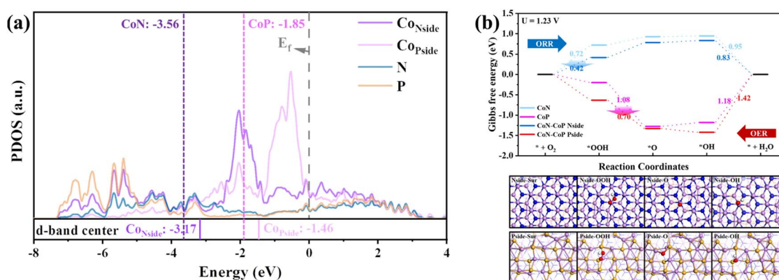
Fig. 5 DFT calculation for CoP/CoN@NCNRs/CC: (a) PDOS calculation, and (b) free energy plot for the ORR and OER on CoN, CoP and CoP/CoN; reaction mechanisms for the OER and ORR on the target-specific N side and P side, respectively.
