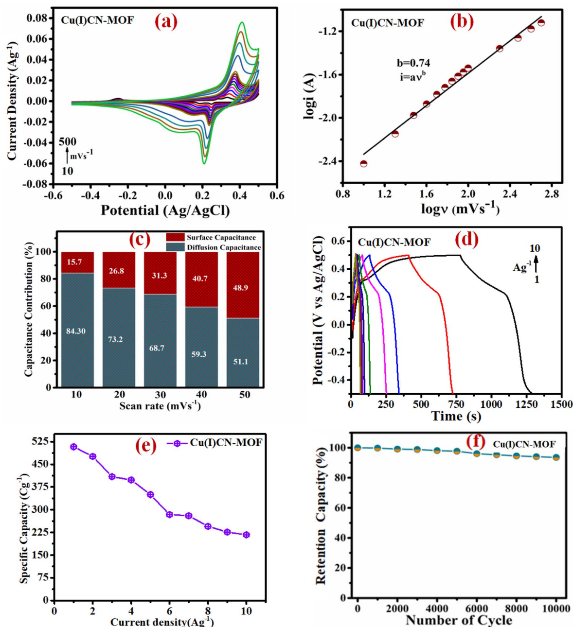
Fig. 5 (a) CV of CuCN-MOF at different scan rates. (b) Charge storage kinetics: \log i vs. \log v plots of CuCN-MOF. The slope of each plot represents the value of b . (c) Percentage surface and diffusion-controlled capacity contributions at different scan rates to the overall capacity of CuCN-MOF. (d) GCD at different current densities of CuCN-MOF. (e) Specific capacity value of CuCN-MOF at different current densities (1–10 A g -1 ). (f) Cyclic stability at 10 A g -1 for 10 000 cycles.
