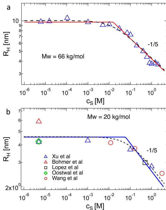
Fig. 31 Hydrodynamic radius of NaPSS in aqueous salt solutions at infinite dilution showing crossover between rod-like and flexible coil. -1/5 Solid lines are fitted to R_H = R_H(0) for c_s < c'_s to R_H = R_H(0)(c_s/c'_s)^{-1/5} at high c_s . Dashed lines are fit to crossover function R_H(c_s) = R_H(0)/(1 + c_s/c'_s)^{-1/5} . The value of R_H at low salt and the cross-over salt concentration ( c'_s ) are left as fitting parameters. Data for panel (a) are from ref. 211 and for panel (b) from ref. 19, 383, 386, 410, 496 and 656. Xu et al. 's values are interpolated.
