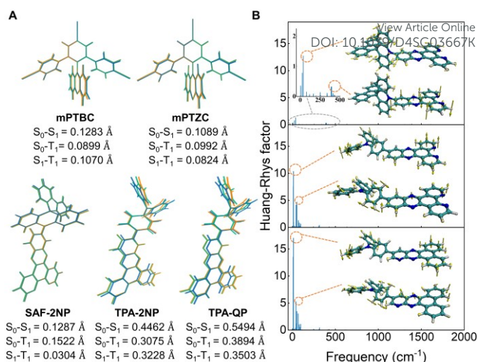
Figure 2. (A) S_0 , S_1 and T_1 (in blue, orange and green, respectively) geometry variations of the five monomers and corresponding RMSD values. (B) Calculated S_0-S_1 Huang-Rhys factors of SAF-2NP (upper), TPA-2NP (middle) and TPA-QP (lower) at different frequencies (insert: representative vibrational modes).
