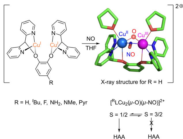
Fig. 10 Synthesis of [R]Cu 2 (μ-O)(μ-NO)] 2+ species and influence of the spin state on HAA reactivity from ref. 73 and 74.
