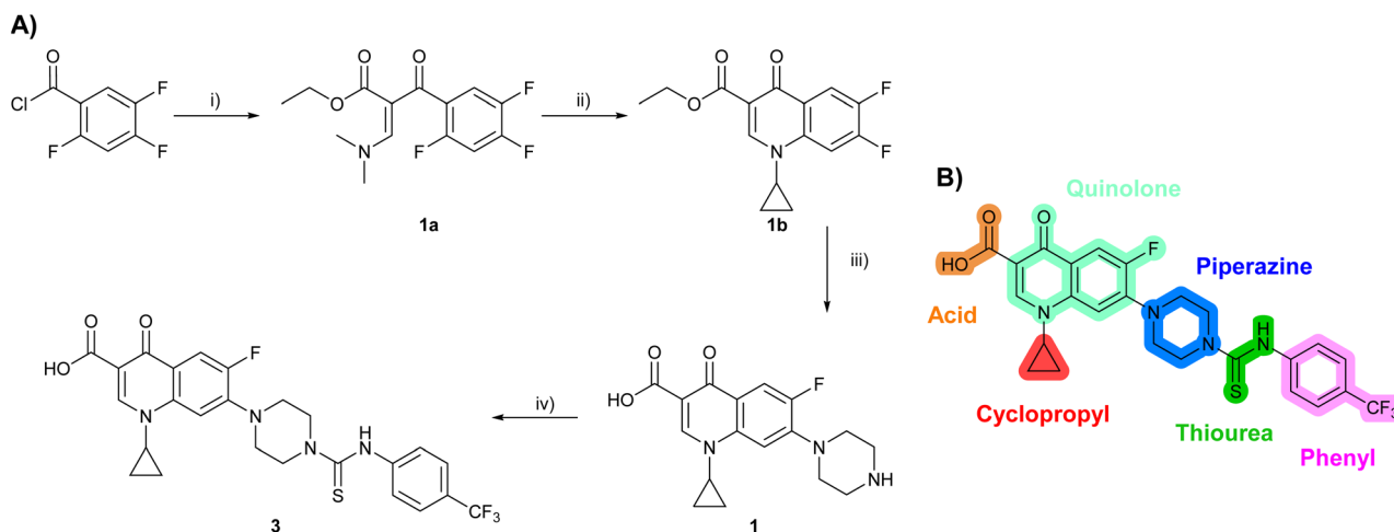
Scheme 1 Synthesis of compounds 1 and 3. (A) Reagents, conditions and yields: (i) ethyl 3-( N,N -dimethylamino)acrylate, Et 3 N, toluene, 80 °C, 20 h (65%); (ii) (a) cyclopropylamine, Et 2 O, EtOH, RT, 3 h. (b) K 2 CO 3 , DMF, 100 °C, 18 h (58%); (iii) (a) piperazine, MeCN, 80 °C, 18 h; (b) NaOH (1 M), 80 °C, 2 h (96%); (iv) 4-(trifluoromethyl)phenyl isothiocyanate, K 2 CO 3 , MeCN, RT, 18 h (92%). (B) Overview of structure-activity relationship (SAR) investigation in this study, with points of variation of 3 colour coded as phenyl (pink), thiourea (green), piperazine (blue), quinolone (turquoise), carboxylic acid (orange), and cyclopropyl (red). Synthetic routes to specific analogues are presented in ESI Schemes S1–S5,† colour coded as in panel (B).
