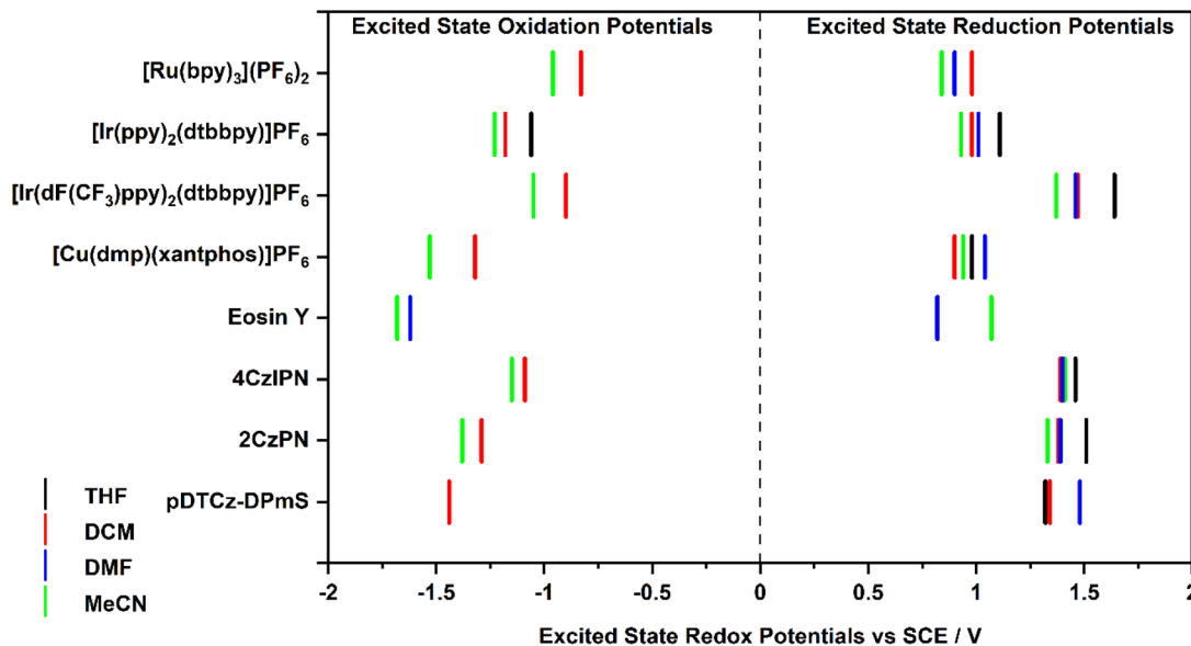
Fig. 7 Summary of the excited-state redox potentials of the eight PCs in the four solvents. Only the E_{\text{ox}}^* based on the first E_{\text{ox}} for [Cu(dmp)(xantphos)]PF 6 in MeCN is provided.
