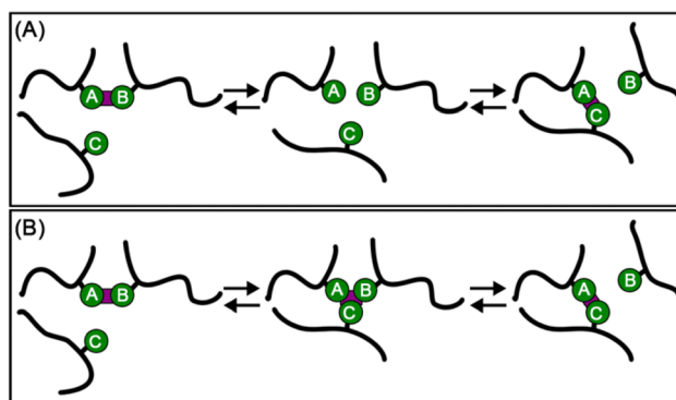
Scheme 1 Mechanisms of cross-link exchange in CANs: (A) dissociative and (B) associative.
