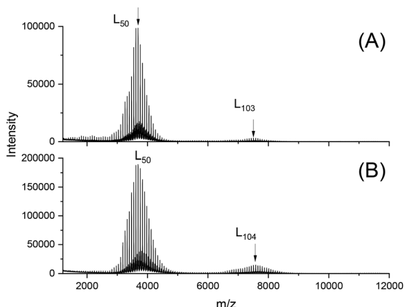
Fig. 6 MALDI-TOF mass spectra of PLAs prepared at 140 °C for 28 d with: (A) SnCl 2 (2D, Table 2); (B) BuSnOPF (4D, Table 2).
