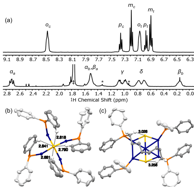
Fig. 2 Top: (a) 1 H NMR spectrum (THF-d 8 , 400 MHz) of 1-dppo showing a conformationally locked ligand configuration about [Cu 12 S 6 ] ( i THF solvent, *residual pentane). Ph o / m / p -CH signals belonging to cisoid versus transoid Ph rings are denoted with c and t subscripts, respectively. Bottom: truncated crystallographic structures of 1-dppo showing CH...S interactions and representative distances with (b) Ph o -CH; (c) α-CH a . Colour scheme: dark grey (cisoid Ph–C); light grey (transoid Ph–C); orange (P); blue (Cu); yellow (S); white (H). H atoms are omitted except cisoid Ph o -CH and octane α-CH a , which are shown interacting with S.
