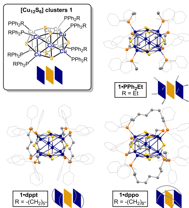
Fig. 1 Structures of [Cu 12 S 6 ] clusters 1 supported by alkyl diphenylphosphine ligands: ball and stick diagrams and cartoon representations of 1-PPh 2 Et (top right), 1-dp (bottom left), and 1-dppo (bottom right) showing ditopic ligand binding mode (adapted from reported crystallographic data 59,61 ). Colour scheme: grey (C); orange (P); blue (Cu); yellow (S). H atoms omitted for clarity. PPh 2 Et: diphenylethylphosphine; dppt: 1,5-bis(diphenylphosphino)pentane; dp: 1,8-bis(diphenylphosphino)octane.
