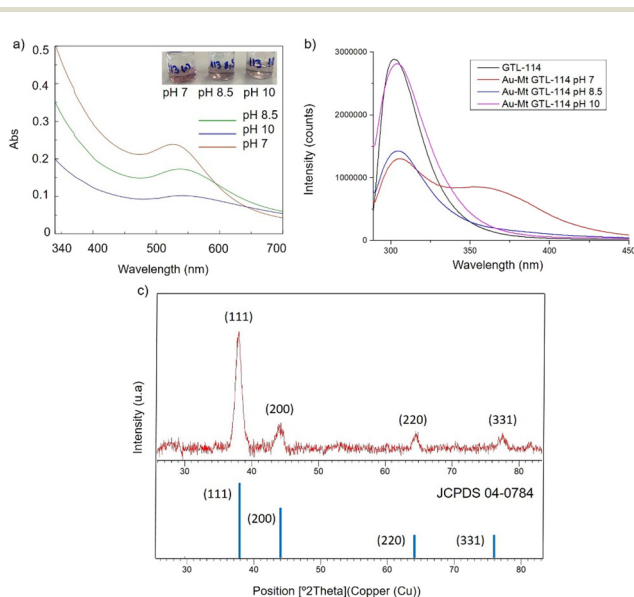
Fig. 2 Characterisation of the different GTL-114 gold metalloenzymes. (a) UV-Absorbance spectrophotometer, (b) fluorescence spectra using 280 nm excitation, (c) XRD pattern.
