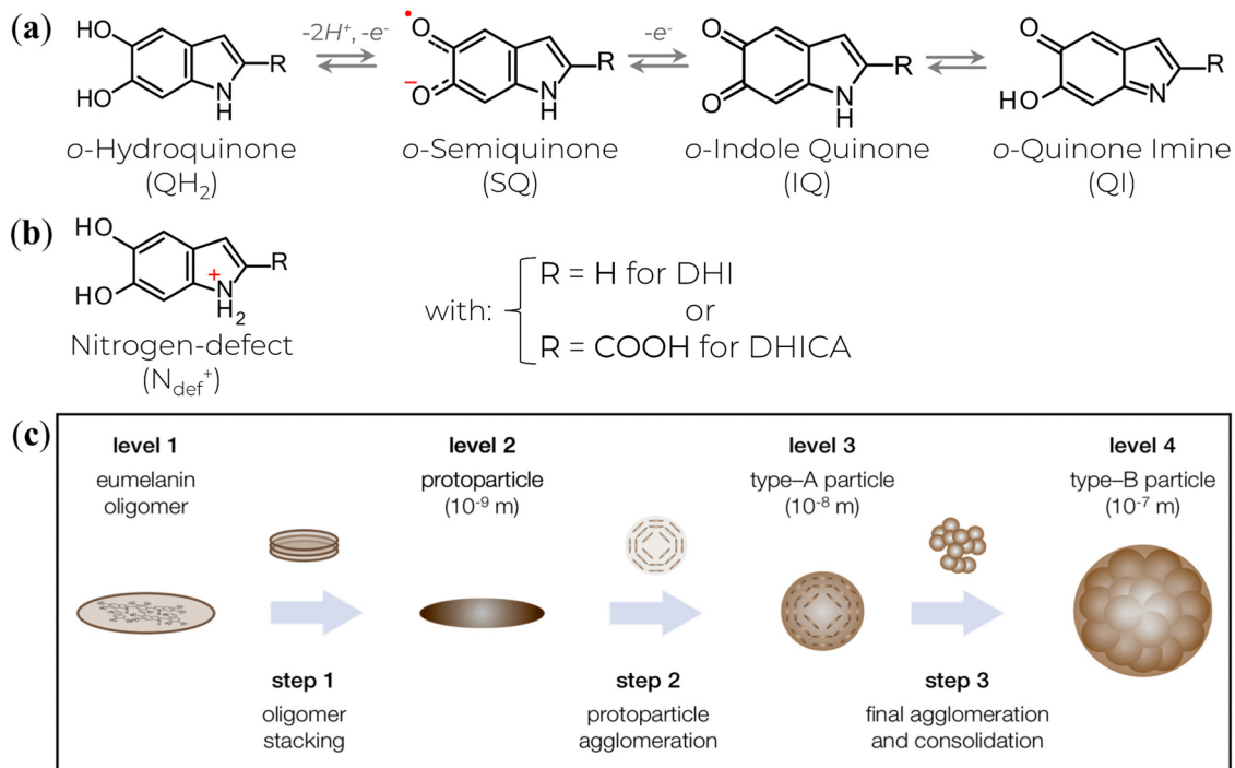
Fig. 1 (a) The various redox states and tautomers of eumelanin monomer building blocks. (b) A charged structure formed during the synthesis and aggregation steps. (c) The current three-step version for eumelanin particle formation. (c) is a reprint from A. Büngeler et al. 49 under Creative Common CC BY license.
