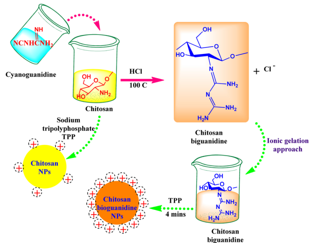
Fig. 1 Ionic gelation method for the synthesis of chitosan biguanidine NPs and unmodified chitosan in the presence of TPP. The cloud of positively charged guanidinium surrounded by chitosan through condensation significantly enhances the antibacterial efficacy.
