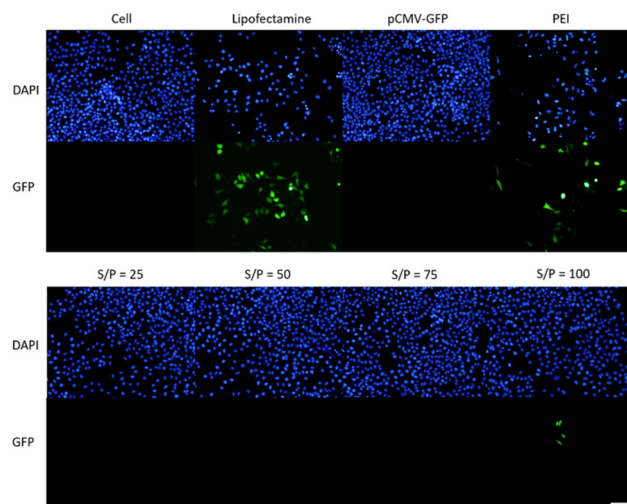
Fig. 14 Fluorescence microscope images of HeLa cells transfected with pCMV-GFP at 0.25 µg per well via 50-THG . Top row depicts the controls: untreated HeLa cells, Lipofectamine™ 3000, plasmid DNA and bPEI 25k at N/P = 25 . 100× magnification. Scale bar represents 200 µm (both top and bottom images).
