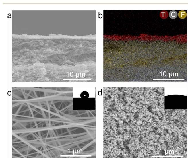
Fig. 2 Structural characterization of the Rh/TiO 2 -GDL. (a) Cross-sectional SEM image and (b) corresponding EDS mapping of Rh/TiO 2 -GDL; top-view SEM images of (c) pristine GDL porous substrate and (d) immobilized Rh/TiO 2 photocatalyst layer. Inserts in (c) and (d) show photographs of water droplets on each sample.
