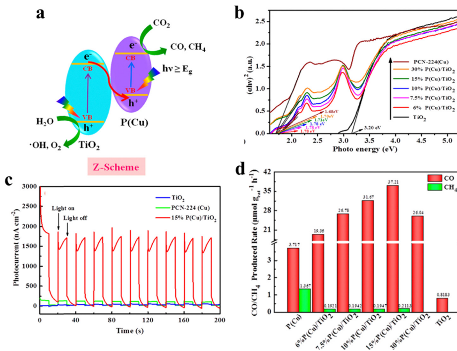
Fig. 14 (a) Direct Z-scheme photocatalytic mechanism. (b) Energy band gaps ( E_g ) of \text{TiO}_2 , \text{PCN-224(Cu)} , and \text{PCN-224(Cu)/TiO}_2 . (c) Photocurrent–time ( I – t ) curves of \text{TiO}_2 , \text{PCN-224(Cu)} , and 15%P(Cu)/ \text{TiO}_2 photoelectrodes at 0.6 V vs. REH bias potential in 0.5 M \text{Na}_2\text{SO}_4 (pH \sim 7.35). (d) CO and \text{CH}_4 generation rate over \text{PCN-224(Cu)} , 6%P(Cu)/ \text{TiO}_2 , 7.5%P(Cu)/ \text{TiO}_2 , 10%P(Cu)/ \text{TiO}_2 , 15%P(Cu)/ \text{TiO}_2 , 30%P(Cu)/ \text{TiO}_2 , and \text{TiO}_2 under 300 W Xe lamps. Reproduced from ref. 64. Copyright 2022 ACS.
