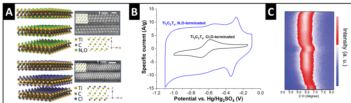
Fig. 5 Solvent cointercalation by tuning nanoconfinement chemistry in MXenes. (A) Structural models and transmission electron micrographs (high-angle annular dark-field) of N,O- and Cl-terminated \text{Ti}_3\text{C}_2\text{T}_x MXenes, (B) their cyclic voltammograms in 3 M \text{H}_2\text{SO}_4 electrolyte at 20 \text{ mV s}^{-1} , and (C) in situ XRD heatmap for two full galvanostatic cycles of the N,O-terminated electrode, replotted or adapted with permission from ref. 51, Copyright 2023 John Wiley & Sons.
