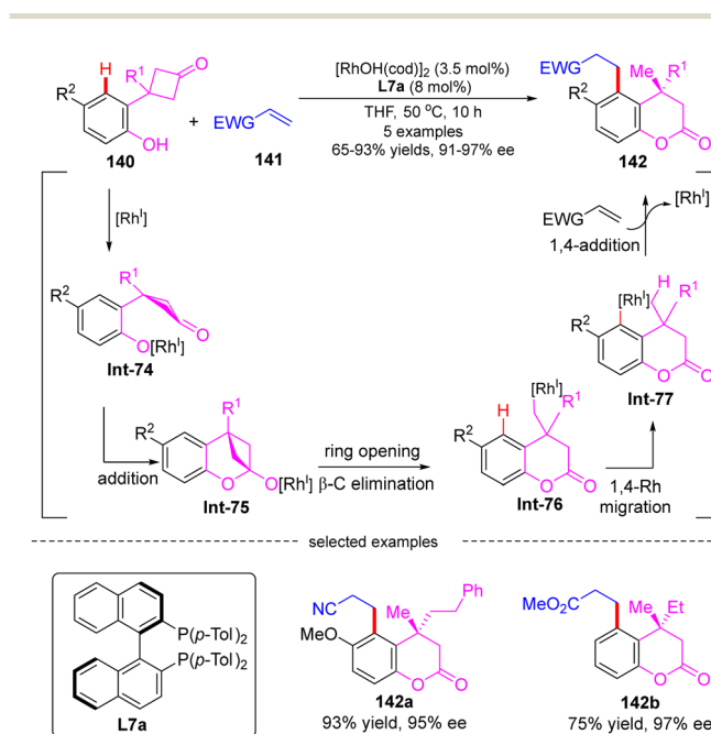
Scheme 39 Rh(I)-Catalyzed arylation of N - or O -tethered alkyne enoates with arylboronic acids.
