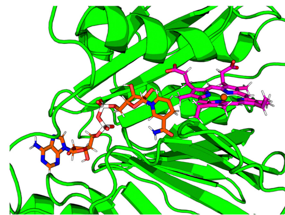
Fig. 8 Top: Close-up representation of the holo -HemS main pocket with NADH (computational reconstruction). NADH is shown in orange. The most important residues implicated in NADH-binding are shown in cyan. Middle: Representative structure of folded NADH docking to the heme-binding cavity. Bottom: Representative structure of unfolded NADH, where it can access heme.
