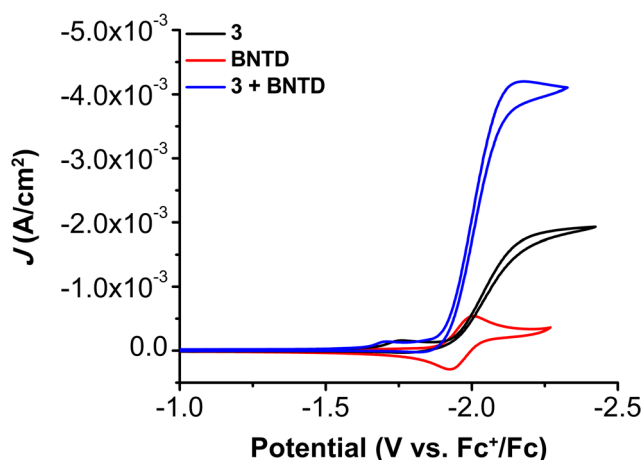
Fig. 3 CVs of 1.0 mM \text{Cr}(\text{tBu-dh}(\text{tBu})\text{bpy})\text{Cl}(\text{H}_2\text{O}) 3 and 2.5 mM BNTD alone and together under \text{CO}_2 saturation conditions with 0.5 M PhOH in DMF demonstrating the shift in catalytic potential.
