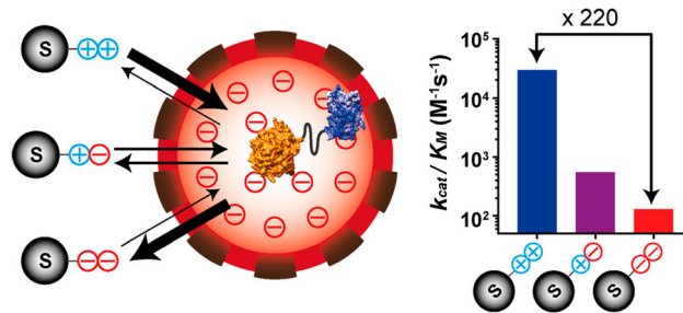
Fig. 5 The access of charged substrates to an enzyme was altered using the highly negatively charged luminal surface of an engineered lumazine synthase protein cage. Reprinted with permission from ref. 42. Copyright 2017 American Chemical Society.
